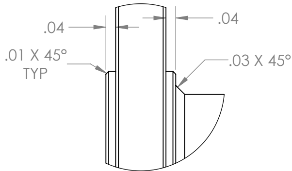
DETAIL A SCALE 3 : 1
