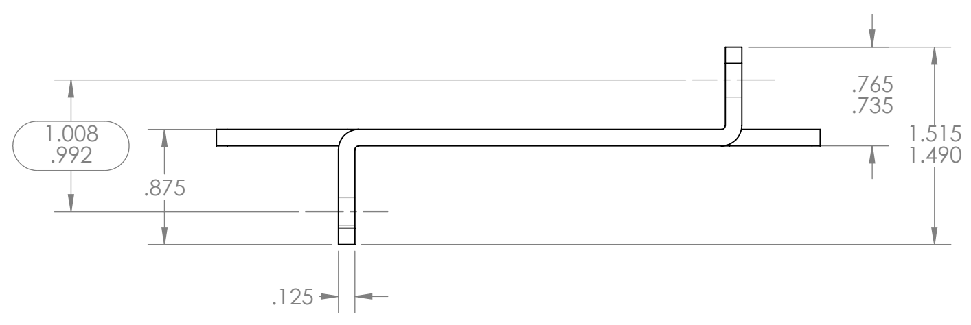
DETAIL A SCALE 1:1
