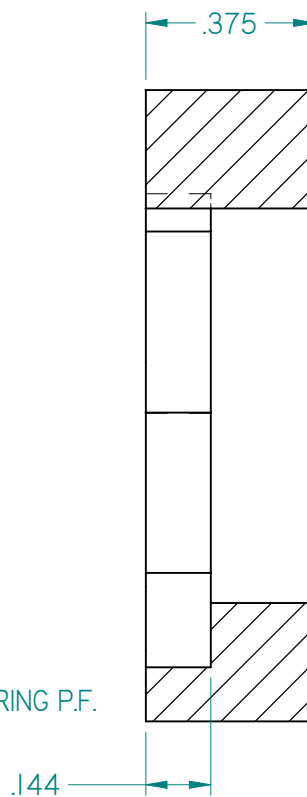
SECTION B-B
