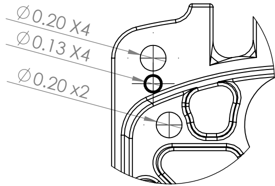
DETAIL A SCALE 2 : 1.5
