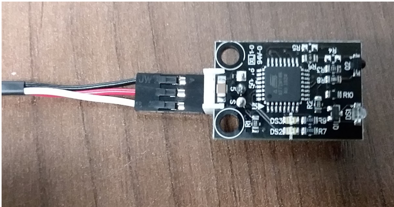
Wiring Photo
