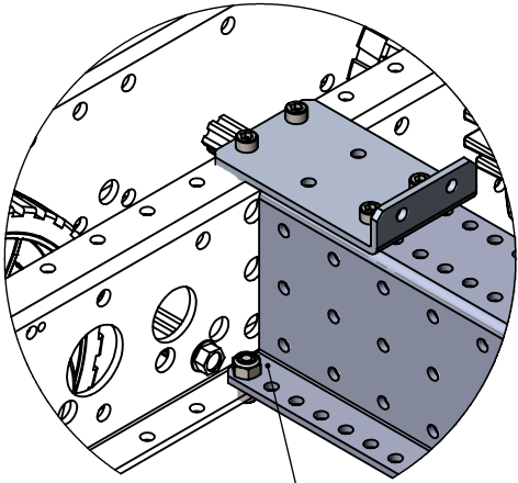
CROSS SHEET ON TOP OF INSIDE FLANGE
