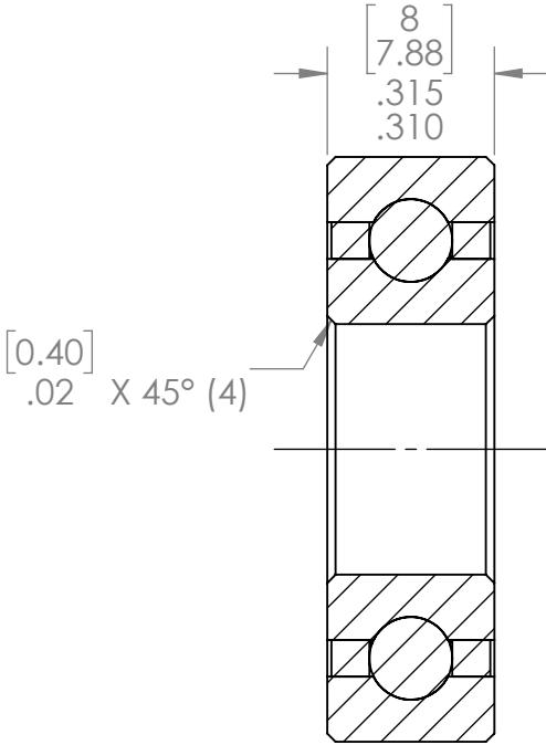
SECTION A-A SCALE 2.5 : 1
