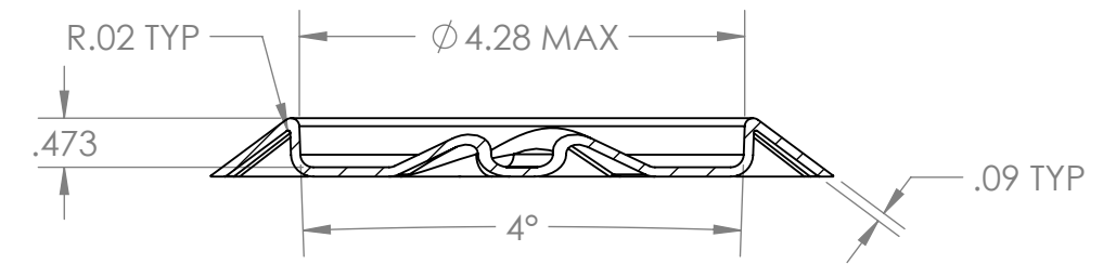
SECTION B-B \curvearrowright 225°
