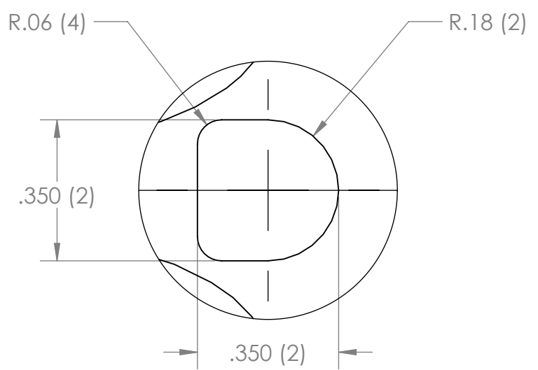
DETAIL C SCALE 3:1
