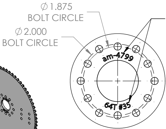
DETAIL B SCALE 1 : 1.5
