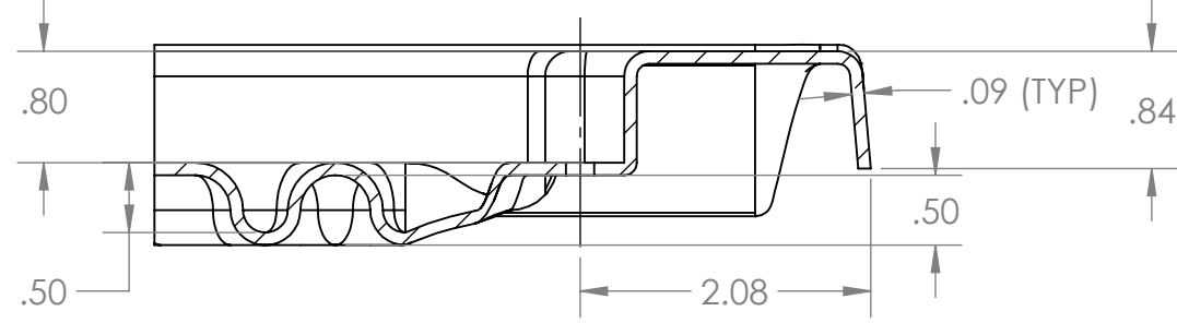
SECTION E-E SCALE 2 : 3
