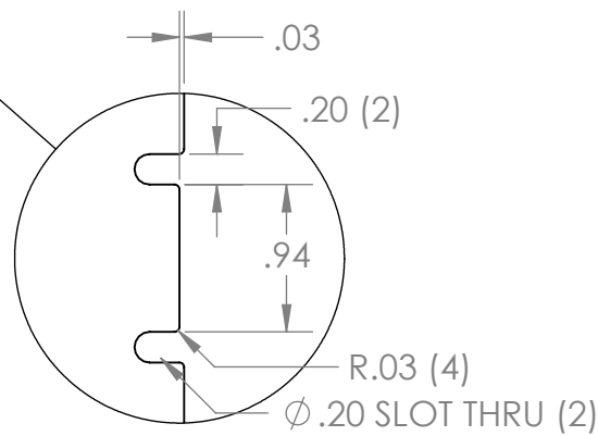
DETAIL B SCALE 3 : 4
