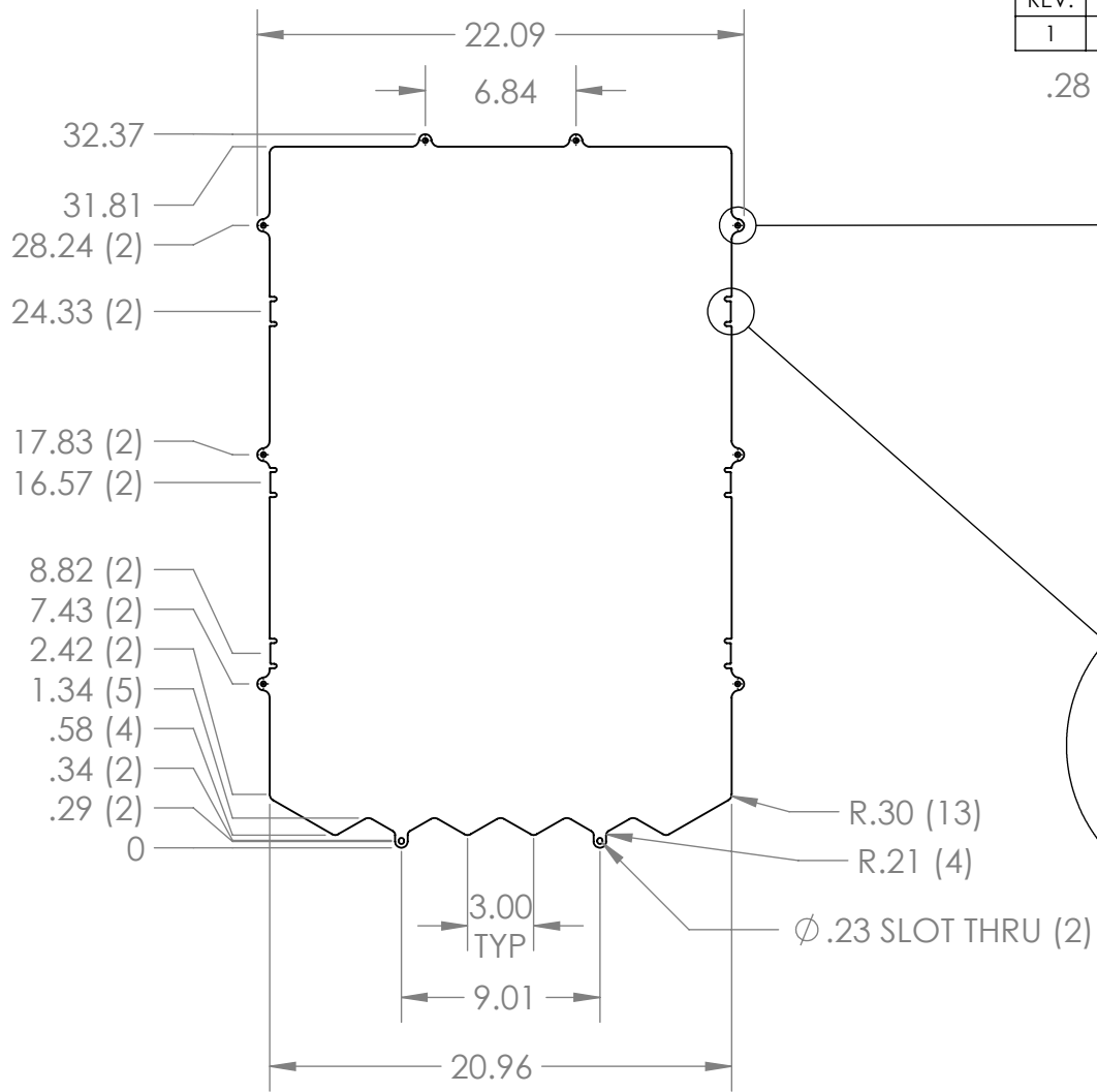
DETAIL A SCALE 3 : 4
