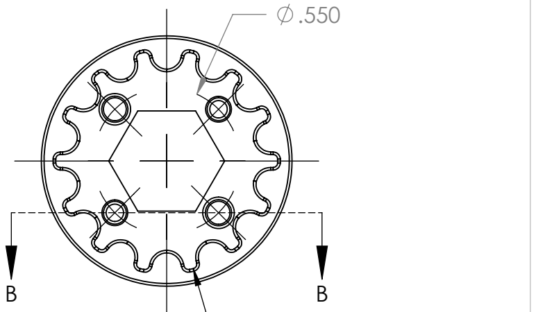
14 TEETH TIMED AS SHOWN 5mm HTD TOOTH PROFILE NO DRAFT
