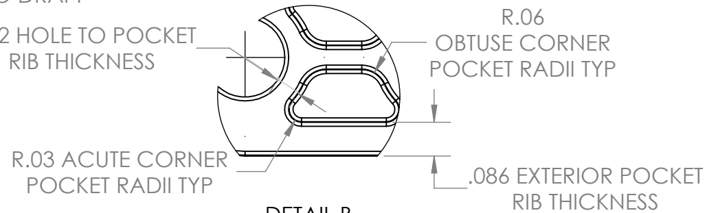
DETAIL B SCALE 3 : 1
