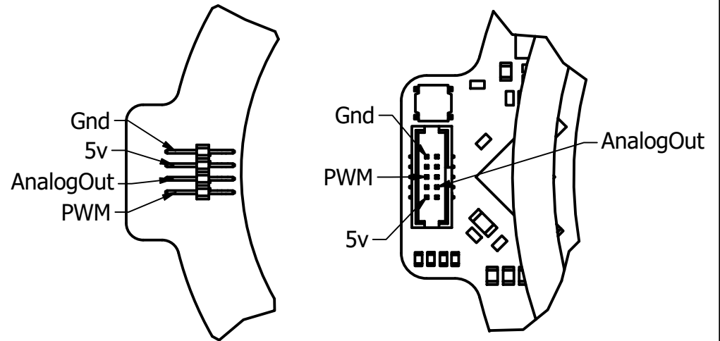
221 Robotic Systems - Lamprey2 4in. Hollow Bore Absolute Encoder
