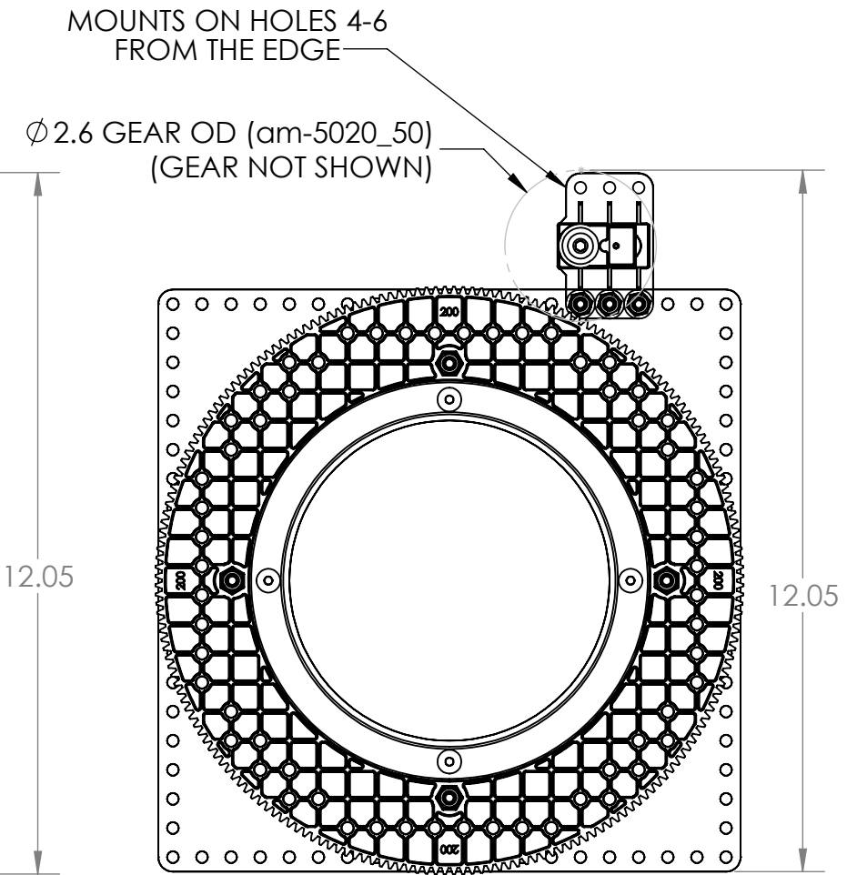
SERVO DRIVE CONFIGURATION
