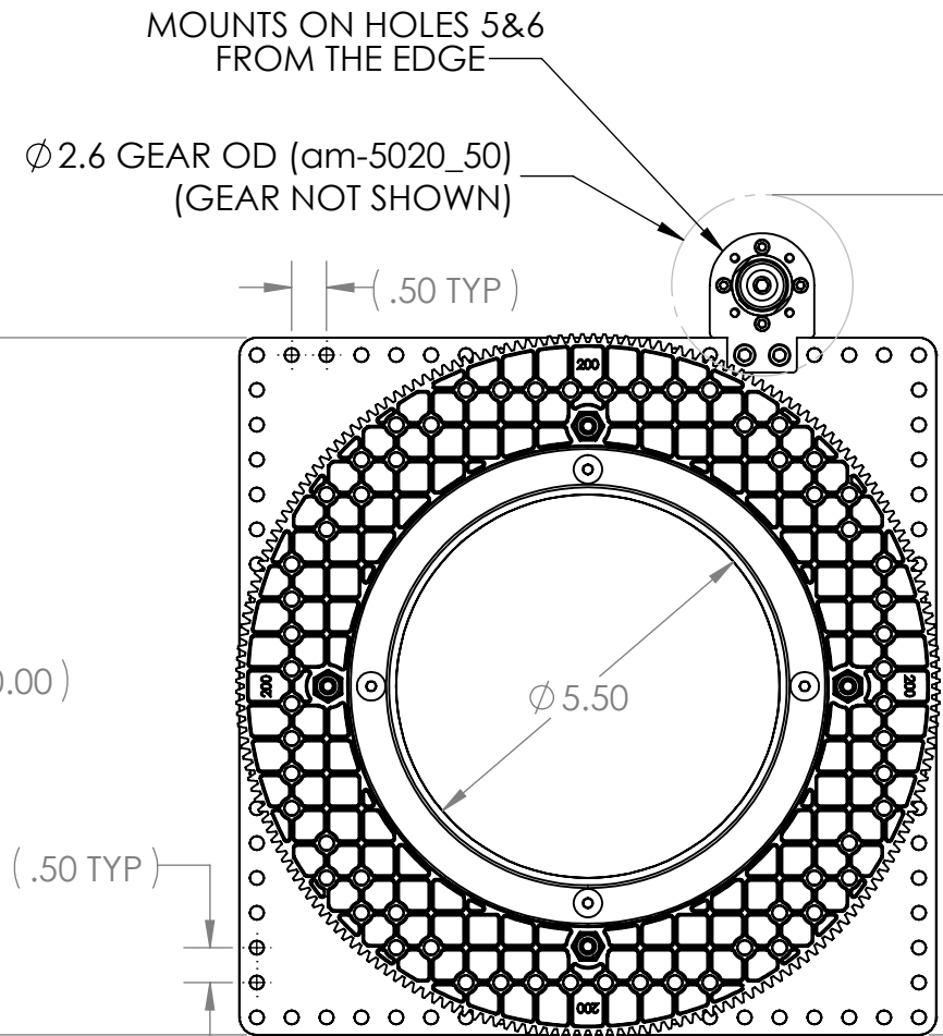
MOTOR DRIVE CONFIGURATION
